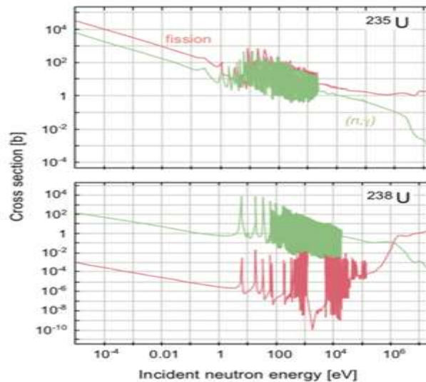
Figure 3 : The fission and neutron absorption cross section in barns (1 barn is 10^{-24} cm) for ^{235}\text{U} and ^{238}\text{U} as a function of the energy of the incident neutron. The cross sections look about the same for all fertile and fissile nuclei, depending whether their atomic number is odd or even.
