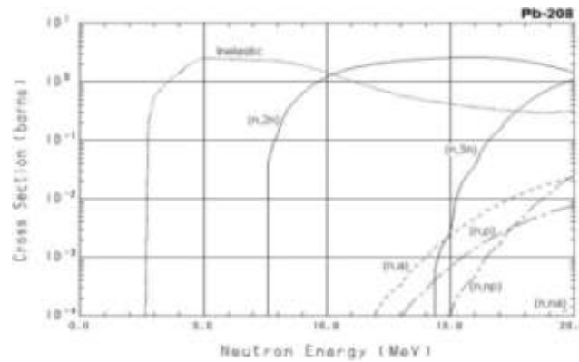
Figure (12). The cross sections for producing 1 or 2 additional neutrons in a lead target, as a function of the incident neutron energy.
